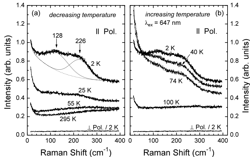
Figure 8. Raman spectra of \text{MgB}_2 at ambient pressure for (a) decreasing and (b) increasing temperatures. ‘|| Pol.’ and ‘ \perp Pol.’ refer to parallel and crossed polarizations of the incident and scattered light, respectively.
