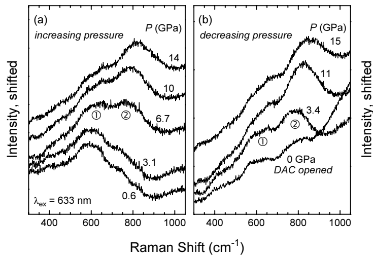
Figure 6. Raman spectra of MgB 2 for (a) increasing and (b) decreasing pressures ( T = 300 K). In between, the pressure was increased to ~20 GPa. After pressure release the sample was in contact with air before the 0 GPa spectrum in (b) was recorded.
